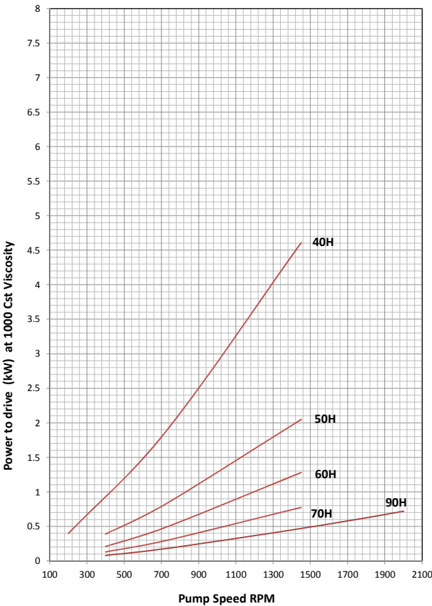
40H - 90H Minimum Facewidth Rotors
